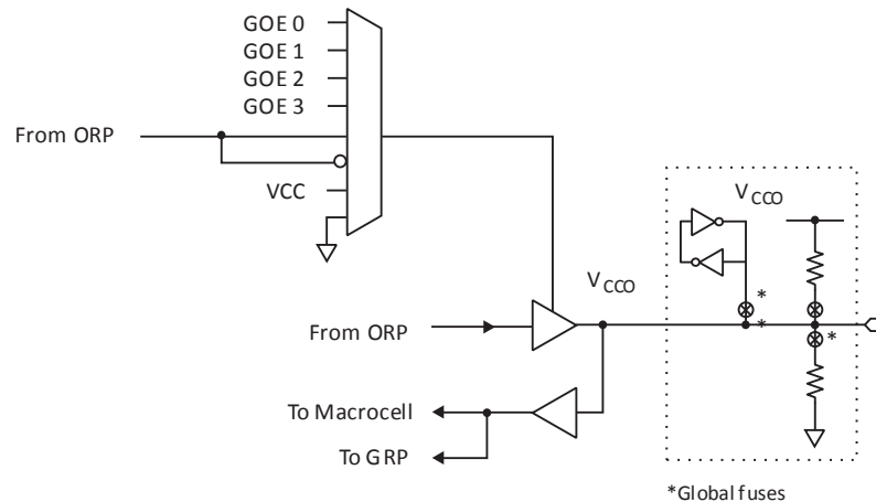
Figure 5.1. I/O Cell
