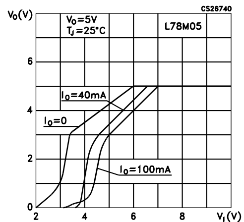
Figure 9. Dropout characteristics
