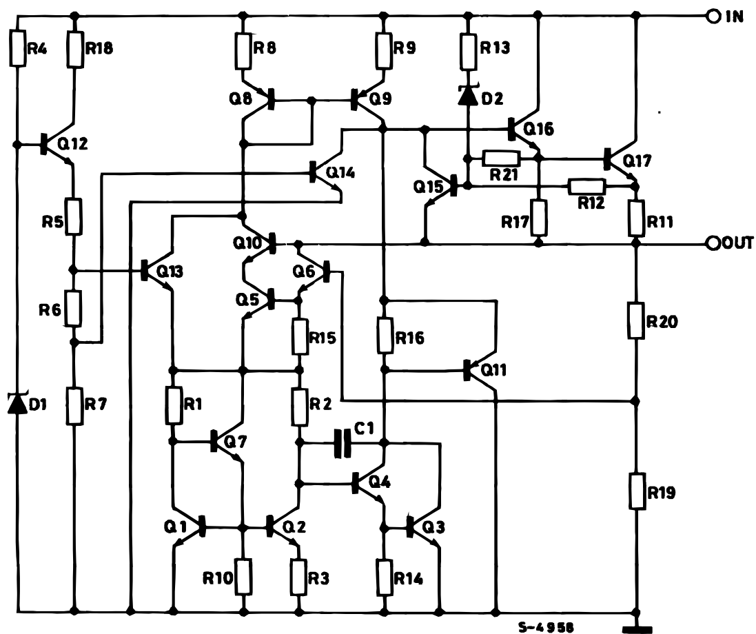
Figure 3. Schematic diagram
