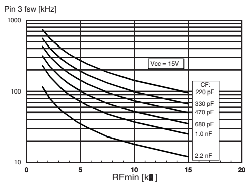
Figure 9. Oscillator frequency vs. timing components
