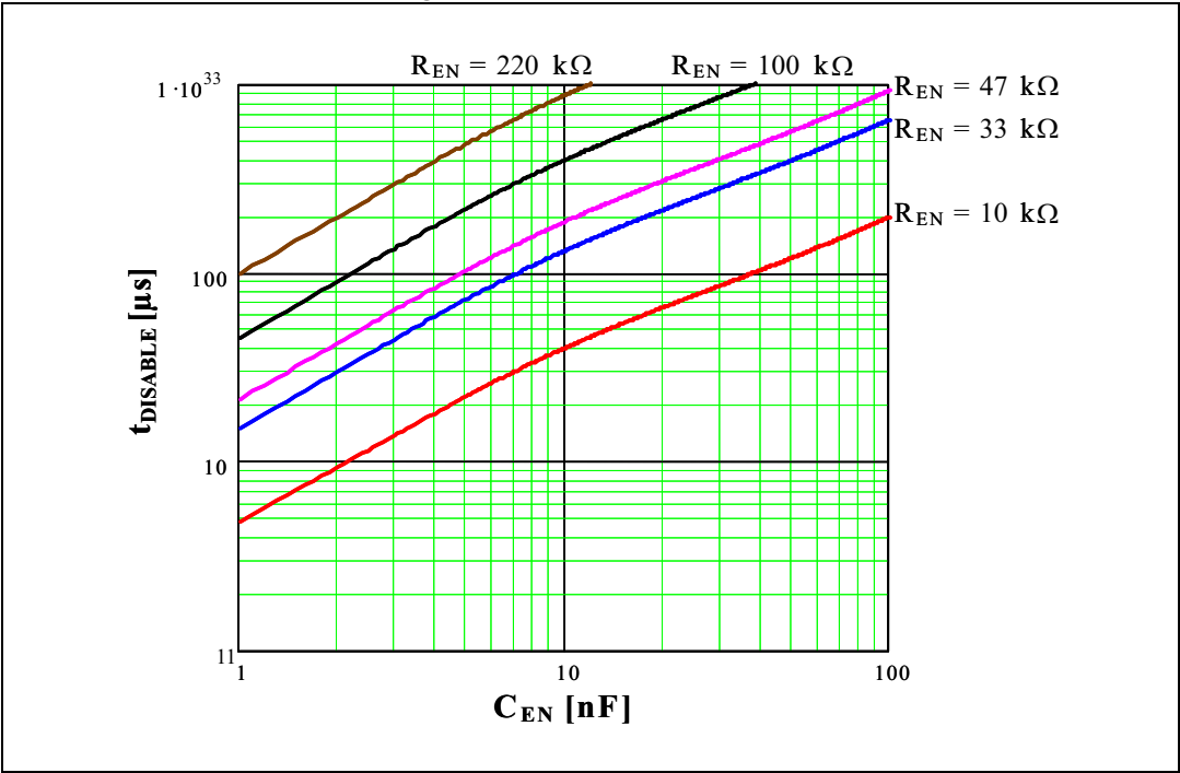
Figure 12. t_{DISABLE} versus C_{EN} and R_{EN} ( V_{DD} = 5\text{ V} )
