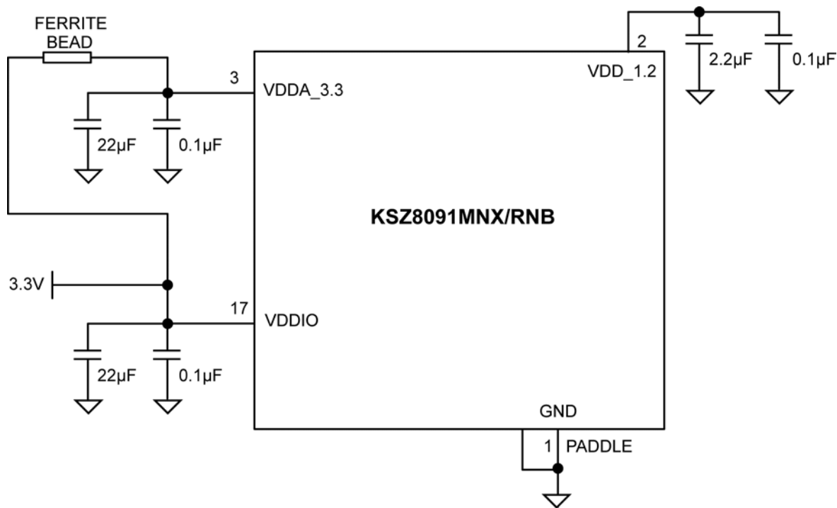
Figure 15. KSZ8091MNX/RNB Power and Ground Connections
