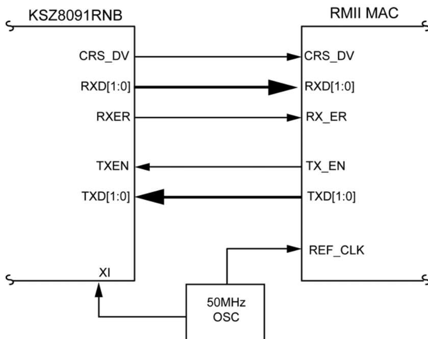
Figure 4. KSZ8091RNB RII Interface (50MHz Clock Mode)
