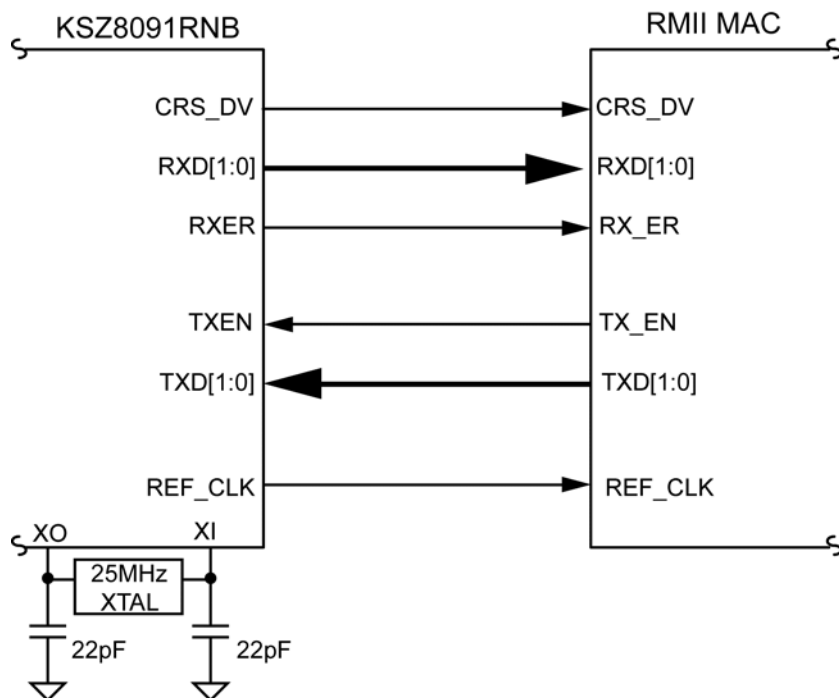
Figure 3. KSZ8091RNB RII Interface (25MHz Clock Mode)
