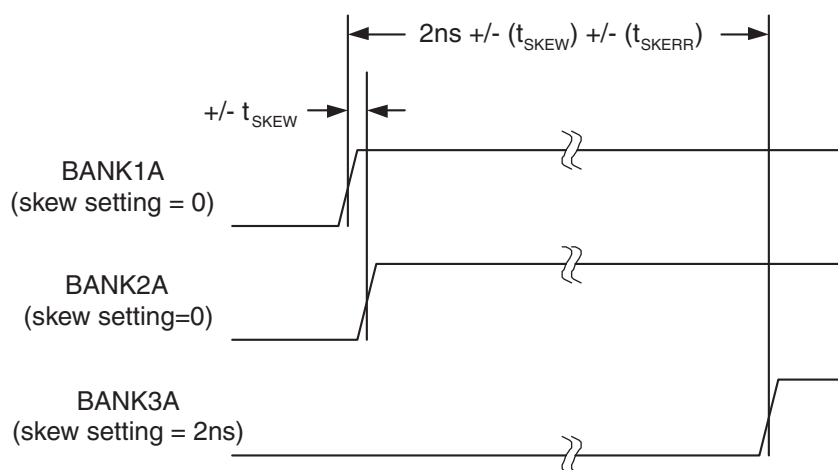
Figure 28. Skew Matching Error Sources
