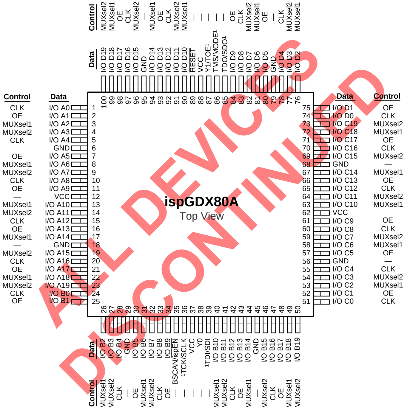
ispGDX80A 100-Pin TQFP Pinout Diagram
