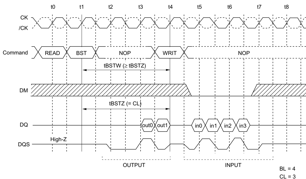
READ to WRITE Command Interval
