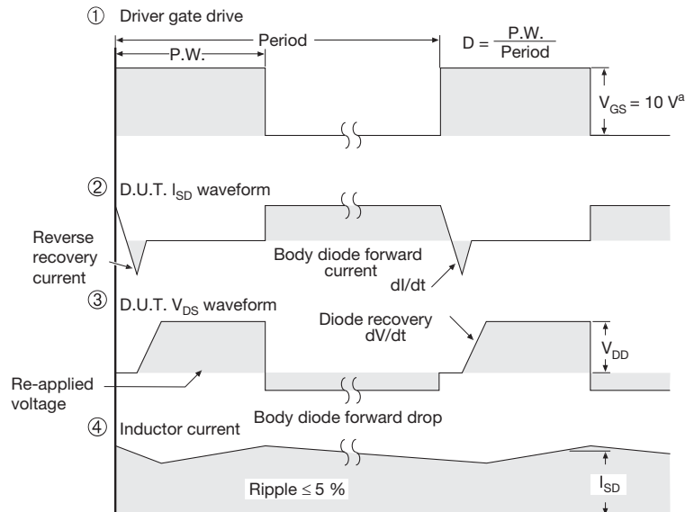
Fig. 14 - For N-Channel
