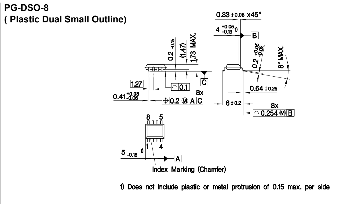
Figure 8 PG-DSO-8-8
