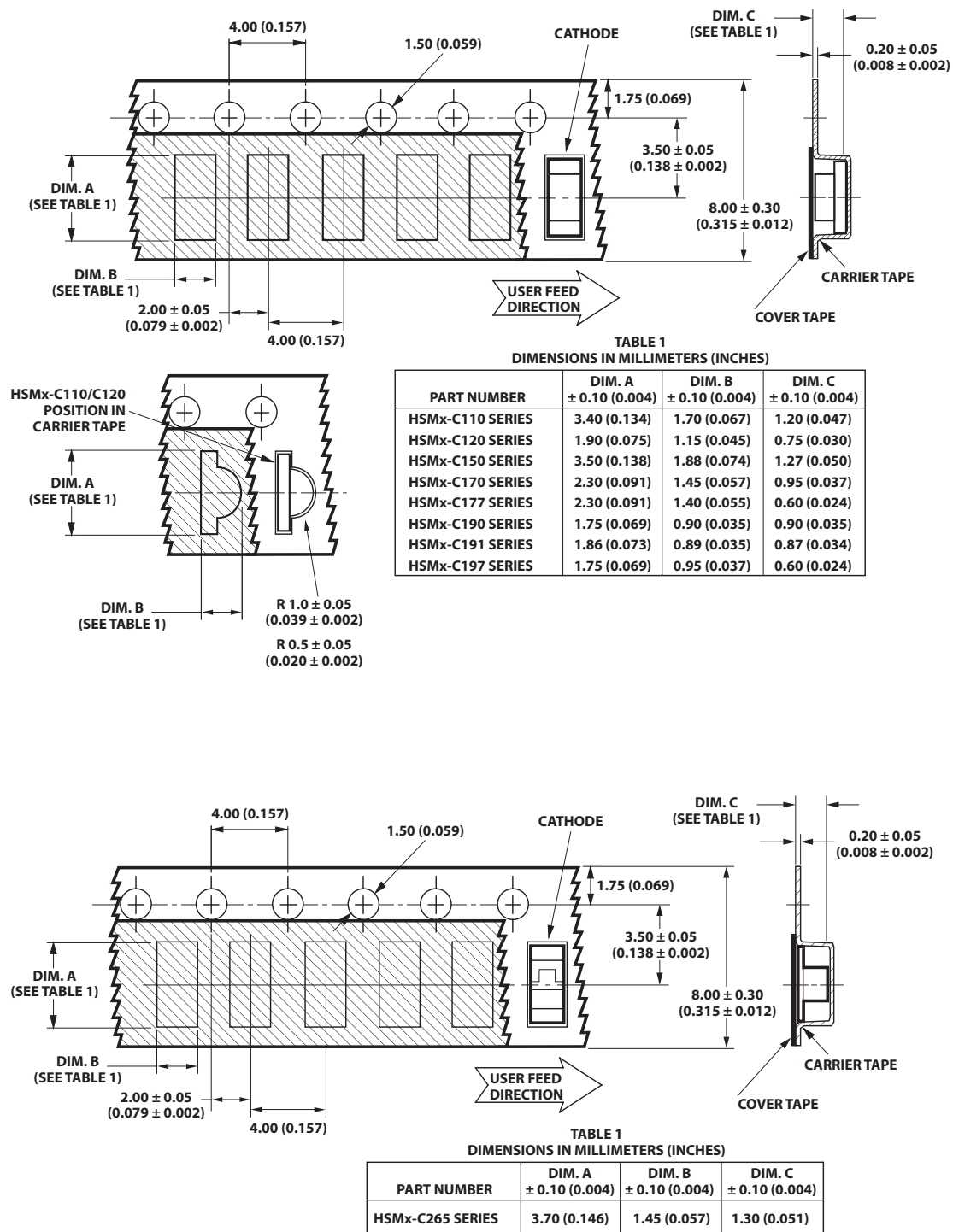
Figure 19. Tape dimensions.
