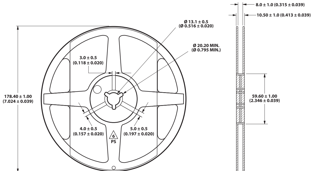
Figure 18. Reel dimensions.
