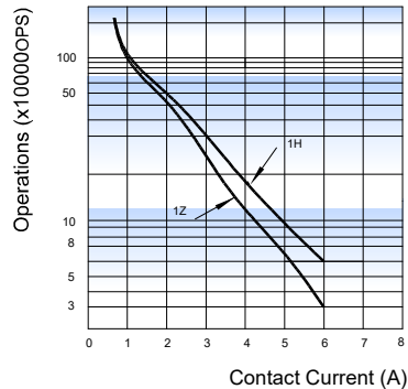
ENDURANCE CURVE
