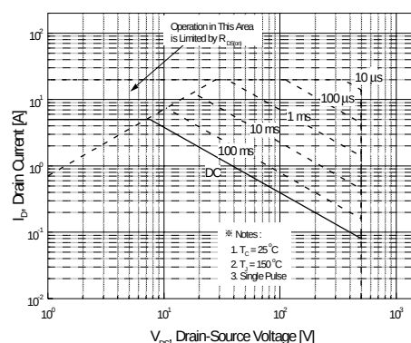
Figure 9-2. Maximum Safe Operating Area for FQPF5N50C
