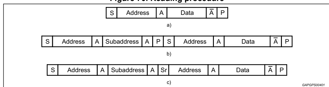
Figure 70. Reading procedure
