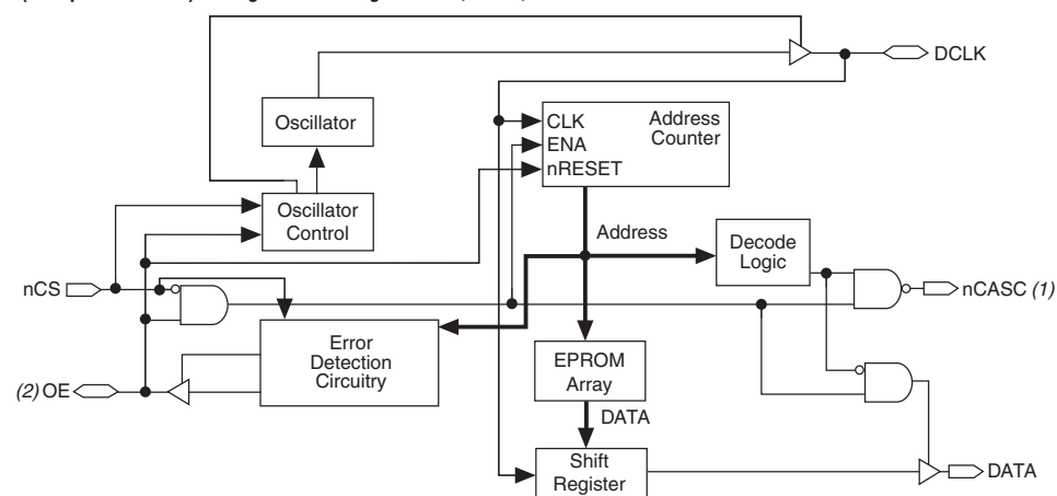
FLEX 8000 Device Configuration Using an EPC1, EPC1441, EPC1213, EPC1064, or EPC1064V
