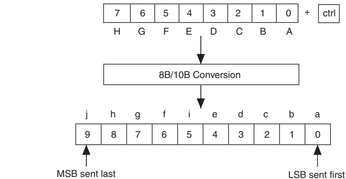
Figure 2–5. 8B/10B Encoding Process
