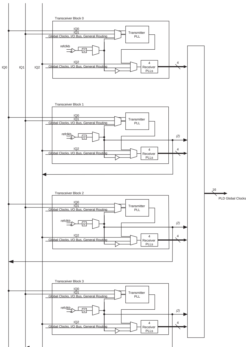
Figure 2–26. EP1SGX25F Device Inter-Transceiver & Global Clock Connections Note (1)
