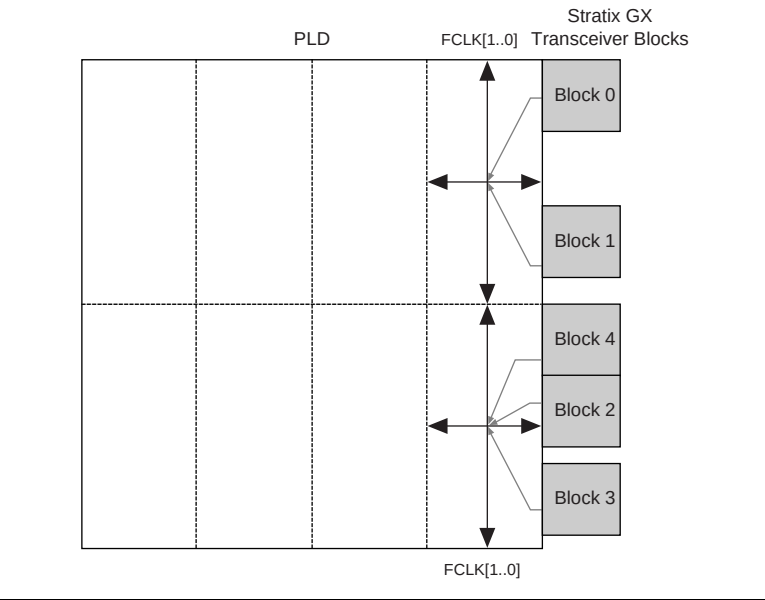
Figure 2–31. EP1SGX40 Receiver PLL Recovered Clock to Fast Regional Clock Connection
