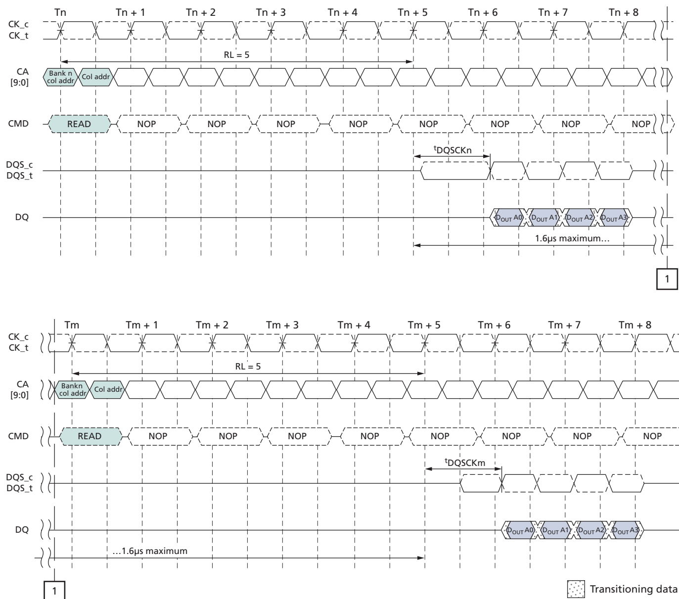
Figure 27: t_{DQSKDM} Timing
