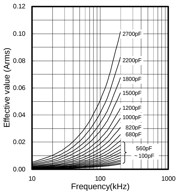
Permissible Current
