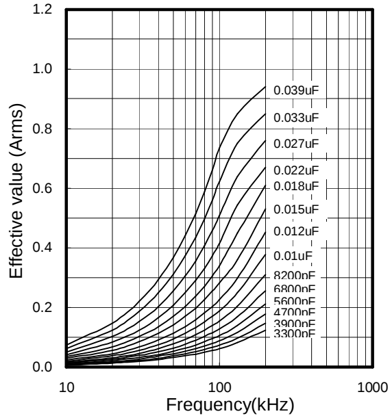
Permissible Current
