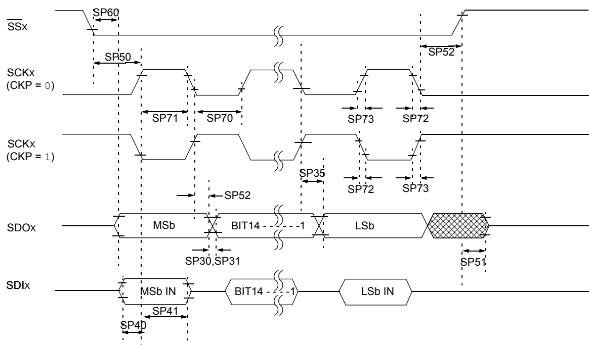
FIGURE 23-17: SPI MODULE SLAVE MODE (CKE = 1) TIMING CHARACTERISTICS
