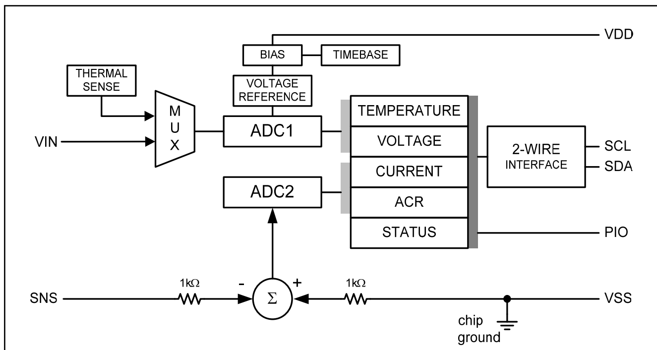
Figure 2. BLOCK DIAGRAM
