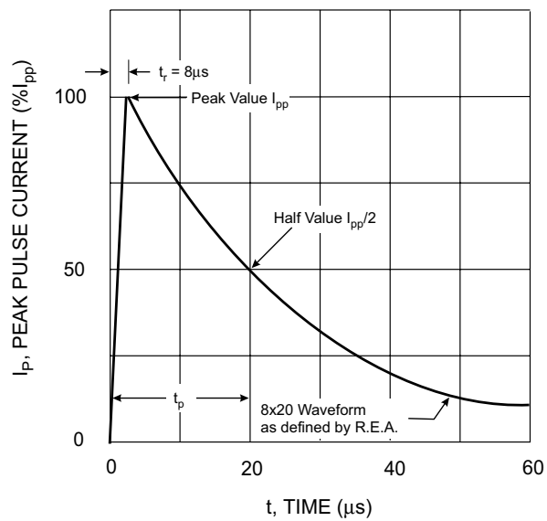
Fig. 4 Pulse Waveform
