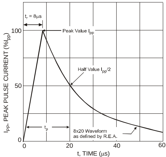
Figure 3 Typical 8 x 20 \mu\text{s} Pulse Waveform
