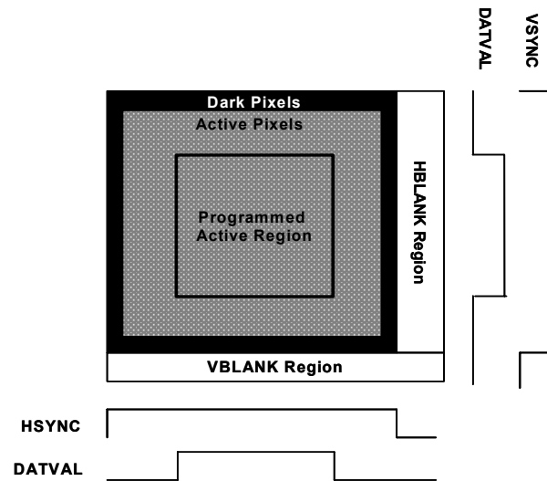
Figure 6-1. Frame Timing
