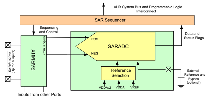
Figure 5. SAR ADC
