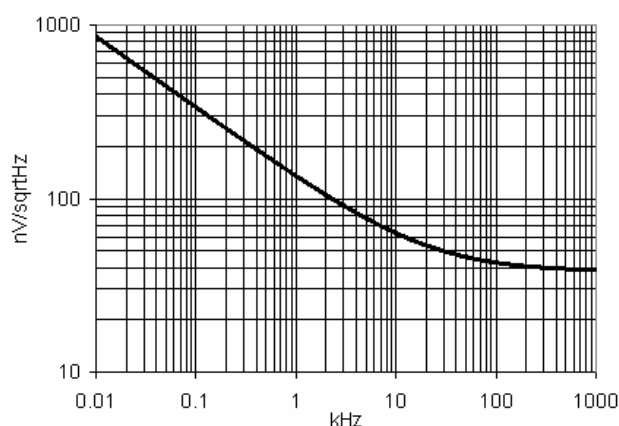
Figure 11-69. Noise vs. Frequency, V DDA = 5 V, Power Mode = High
