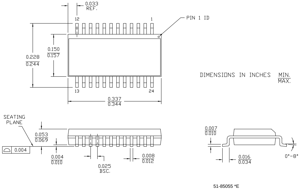
Figure 34. 24-pin QSOP (8.65 × 3.9 × 1.44 mm) O241 Package Outline, 51-85055
