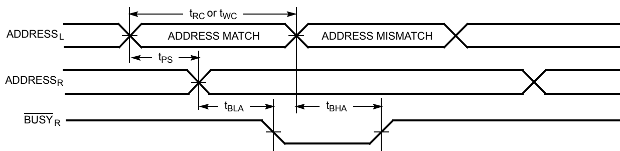
Figure 14. Busy Timing Diagram No.2 (Address Arbitration) [45]
