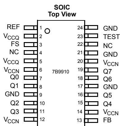
Figure 1. 24-pin SOIC pinout
