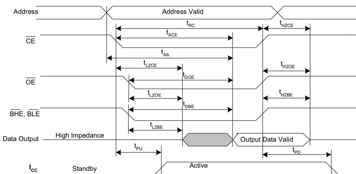
Figure 7. SRAM Read Cycle No. 2 ( \overline{\text{CE}} and \overline{\text{OE}} Controlled) [26, 28, 29]
