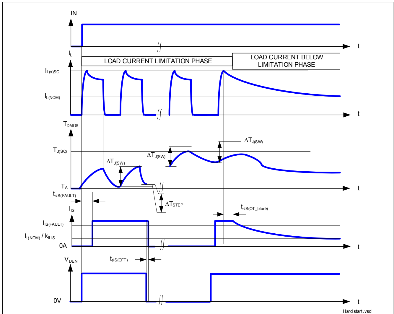
Figure 19 Overload Protection
