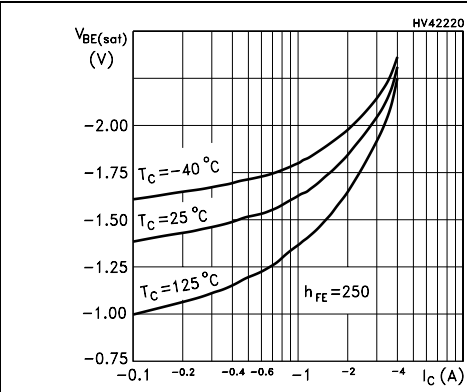
Figure 11. Base-emitter voltage (PNP)
