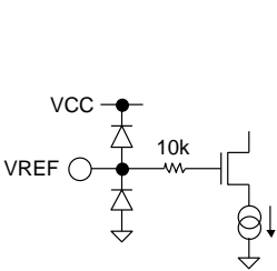
Figure 41. VREF
