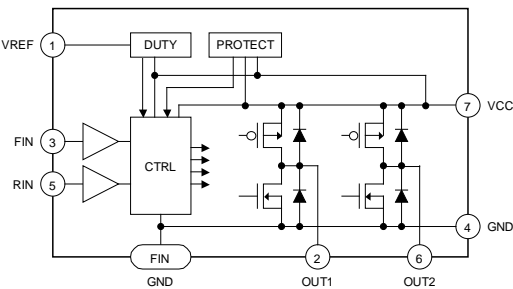
Figure 3. BD6222HFP
