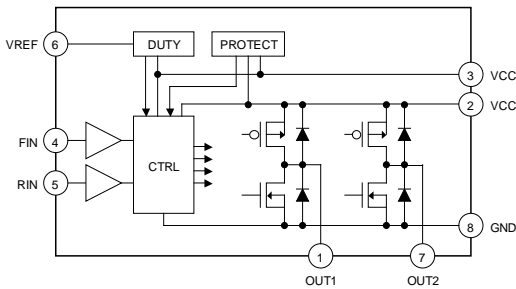
Figure 1. BD6220F / BD6221F
