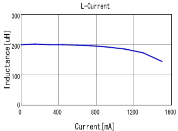
#B966BS-221M=P3 L-Current 20degC
