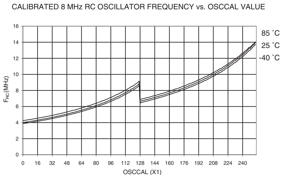
Figure 21-42. Calibrated 8 MHz RC Oscillator Frequency vs. OSCCAL Value
