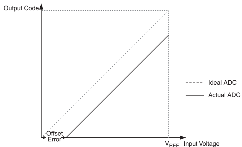
Figure 4-67. Offset Error
