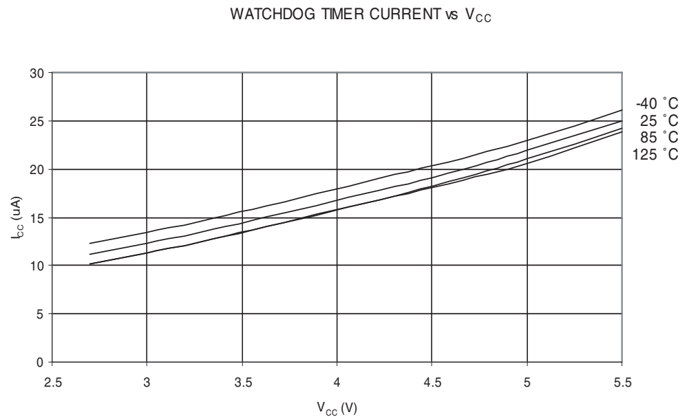
Figure 8-36. Watchdog Timer Current vs. V_{CC}
