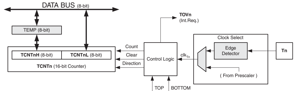
Figure 4-38. Counter Unit Block Diagram
