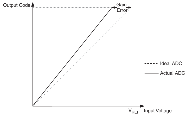
Figure 4-68. Gain Error
