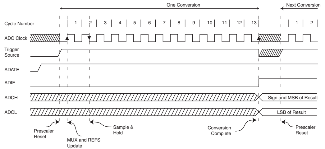
Figure 4-64. ADC Timing Diagram, Auto Triggered Conversion
