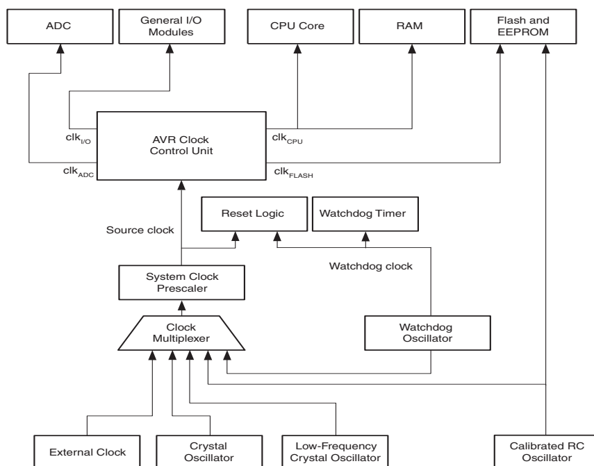
Figure 4-10. Clock Distribution
