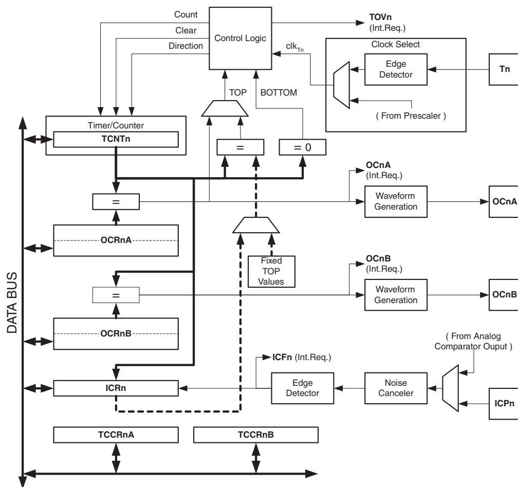
Figure 4-37. 16-bit Timer/Counter Block Diagram
