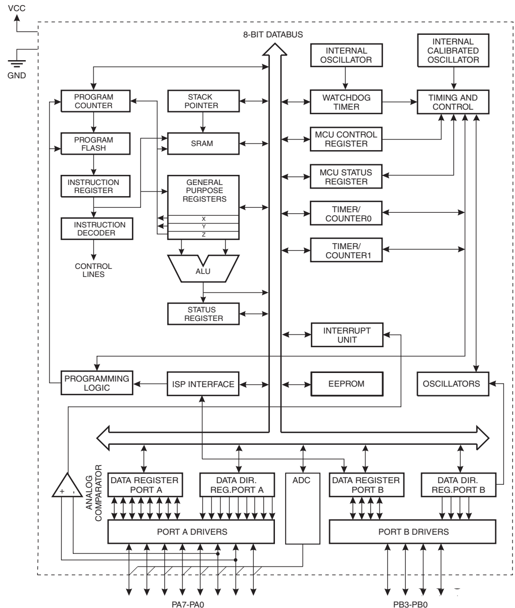
Figure 4-1. Block Diagram
