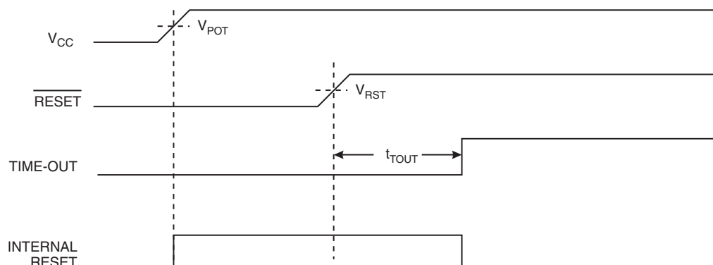
Figure 4-15. MCU Start-up, \overline{\text{RESET}} Extended Externally
