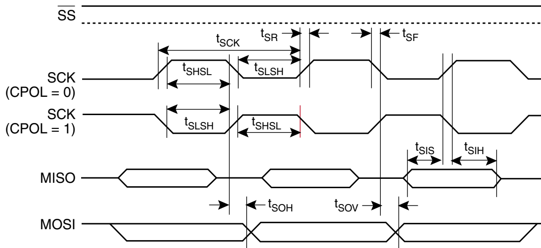
Figure 14-4. SPI Master Timing (CPHA = 0)
