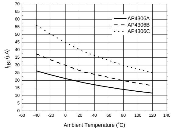
AP4306 I_{BI} vs. Ambient Temperature
