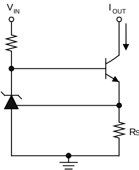
Fig. 7 Constant-Current Sink
