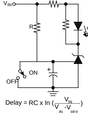
Fig. 5 Delay Timer
