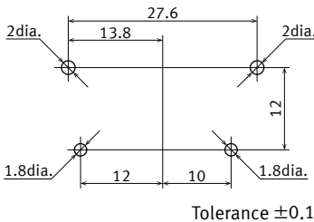
Recommended PC board pattern (BOTTOM VIEW)
