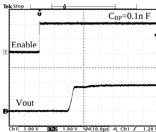
Fig. 20 Start-up Waveform
