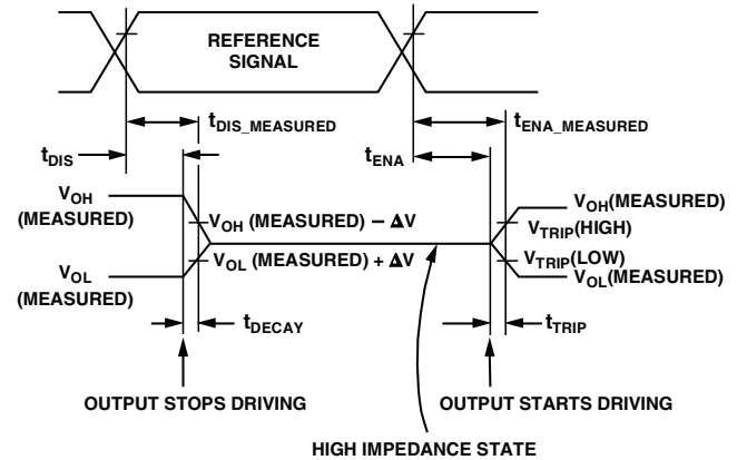
Figure 46. Output Enable/Disable
