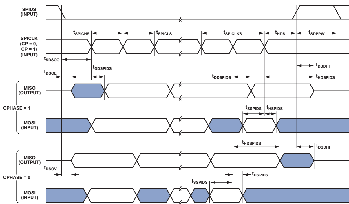
Figure 35. SPI Slave Timing
