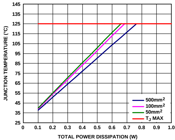
Figure 58. TSOT, T A = 25°C
