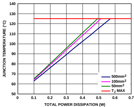
Figure 59. TSOT, T A = 50°C
