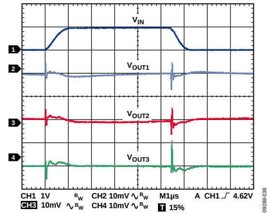
Figure 45. Line Transient Response, V_{IN} = 4 \text{ V} to 5 \text{ V} , I_{LOAD1} = I_{LOAD2} = I_{LOAD3} = 100 \text{ mA} , CH1 = V_{IN} , CH2 = V_{OUT1} , CH3 = V_{OUT2} , CH4 = V_{OUT3} , V_{RIPPLE} = 50 \text{ mV} , C_{OUT} = 1 \mu\text{F}
