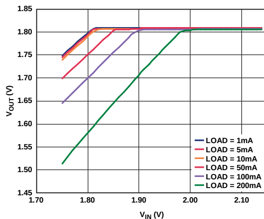
Figure 28. Output Voltage vs. Input Voltage (in Dropout), V_{\text{OUT2}} = 1.8 \text{ V} , V_{\text{RIPPLE}} = 50 \text{ mV} , C_{\text{OUT}} = 1 \mu\text{F}
