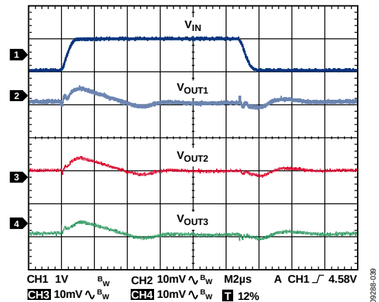
Figure 46. Line Transient Response, V_{IN} = 4 \text{ V} to 5 \text{ V} , I_{LOAD1} = I_{LOAD2} = I_{LOAD3} = 1 \text{ mA} , CH1 = V_{IN} , CH2 = V_{OUT1} , CH3 = V_{OUT2} , CH4 = V_{OUT3} , V_{RIPPLE} = 50 \text{ mV} , C_{OUT} = 1 \mu\text{F}
