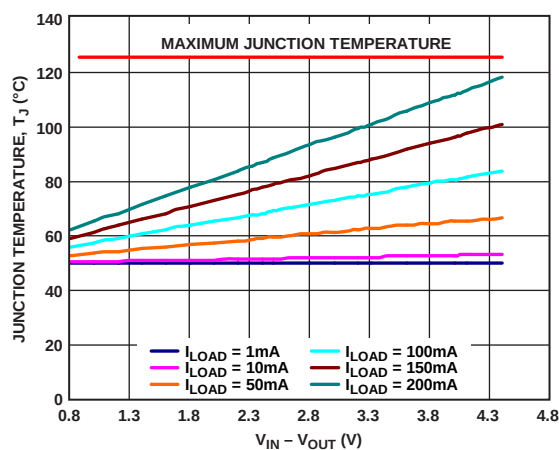
Figure 53. 500 mm 2 of PCB Copper, LFCSP, T_A = 50^\circ\text{C}
