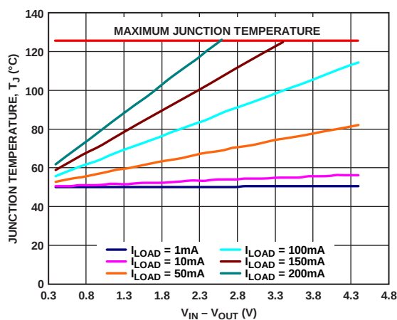
Figure 50. 100 mm 2 of PCB Copper, TSOT, T_A = 50^\circ\text{C}
