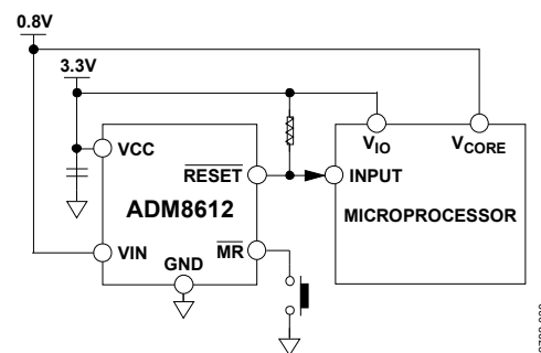
Figure 31. ADM8612 Typical Application Circuit
