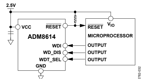
Figure 33. ADM8614 Typical Application Circuit
