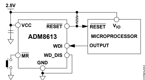
Figure 32. ADM8613 Typical Application Circuit
