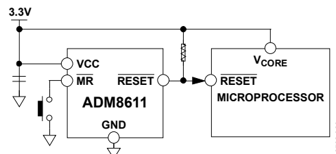
Figure 30. ADM8611 Typical Application Circuit
