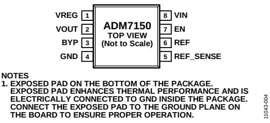
Figure 4. 8-Lead SOIC Pin Configuration
