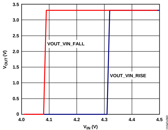
Figure 60. Typical UVLO Hysteresis, V_{OUT} = 3.3\text{ V}
