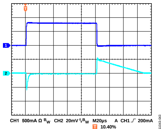
Figure 43. Load Transient Response, I_{LOAD} = 1 \text{ mA} to 800 mA, V_{OUT} = 5 \text{ V} , V_{IN} = 6.2 \text{ V} , CH1 = I_{OUT} , CH2 = V_{OUT}
