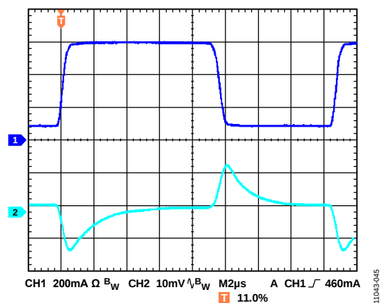
Figure 45. Load Transient Response, I_{LOAD} = 100 \text{ mA} to 600 mA, V_{OUT} = 5 \text{ V} , V_{IN} = 6.2 \text{ V} , CH1 = I_{OUT} , CH2 = V_{OUT}
