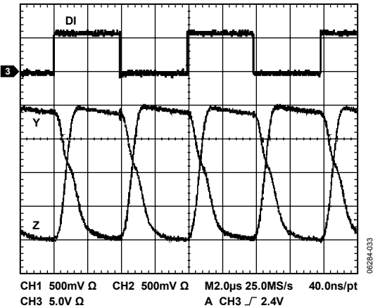
Figure 28. ADM3483E/ADM3488E Driver Propagation Delay
