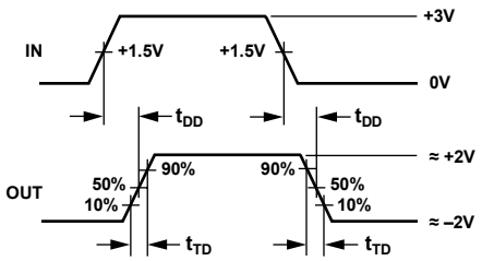
Figure 10. Driver Differential Output Delay and Transition Times
