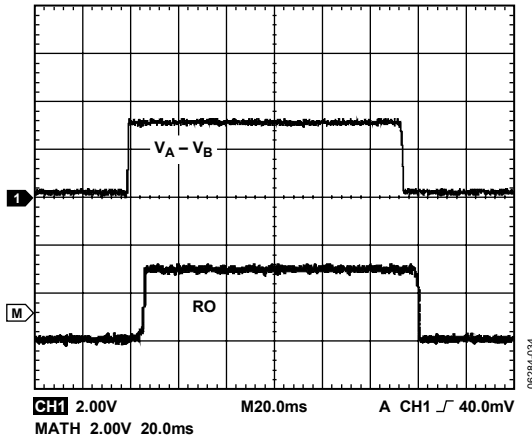
Figure 29. ADM3483E/ADM3488E Receiver Propagation Delay
